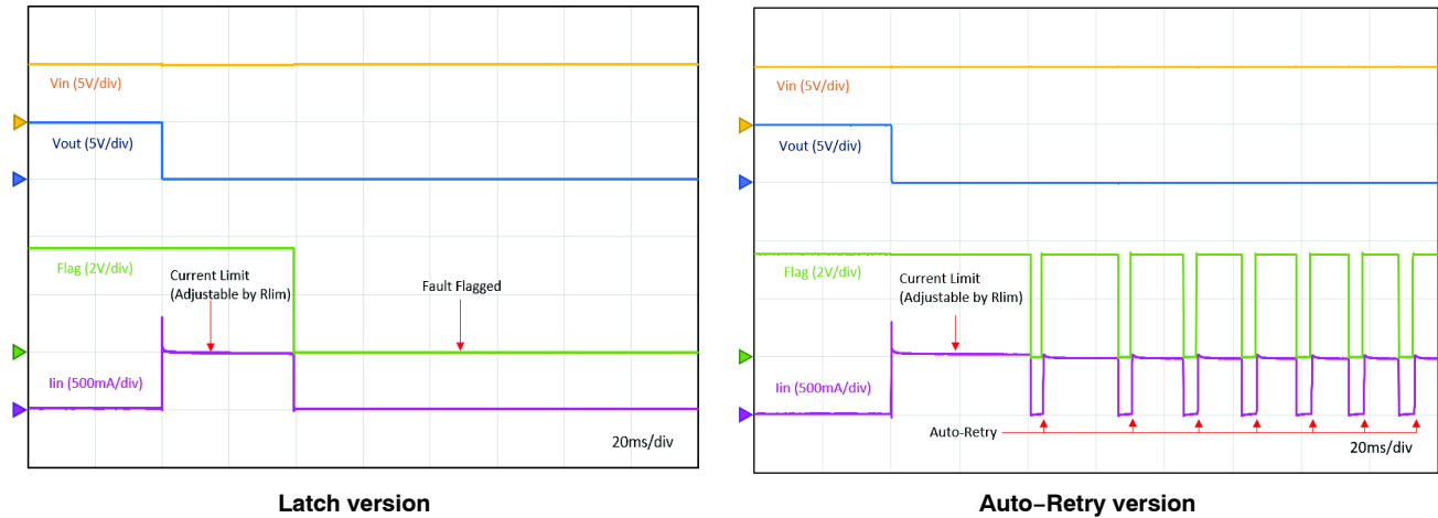
Figure 4. Output Short Circuit
