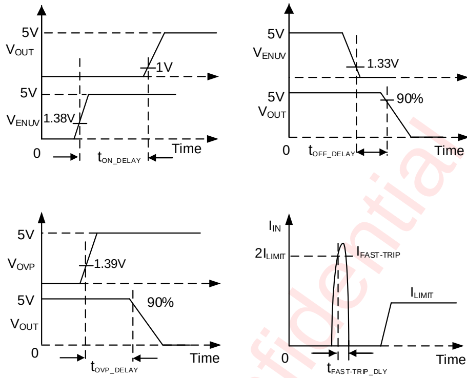
Figure 5 Timing Diagram
