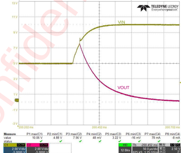
Figure 23 Turn off Delay and Fall Time 150 \mu F // 2.5 \Omega
