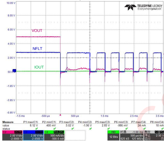
Figure 28 Pulse overvoltage with 100 \Omega
