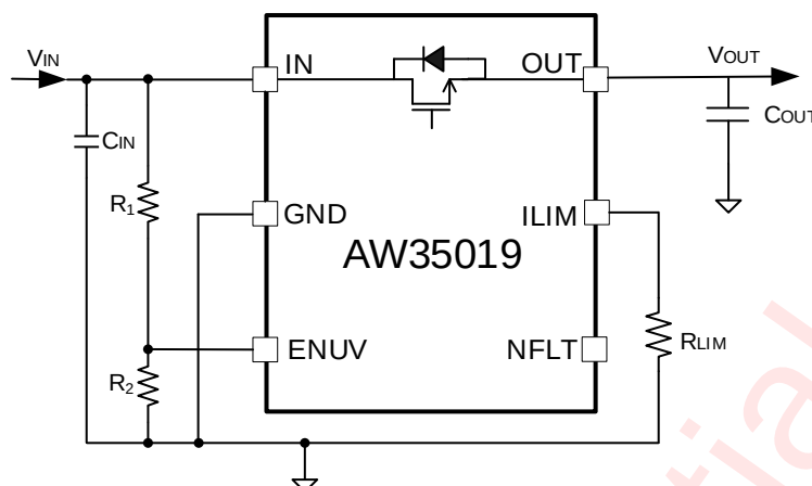
Figure 4 Application circuit
