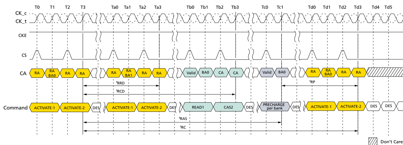
Figure 12: ACTIVATE Command
