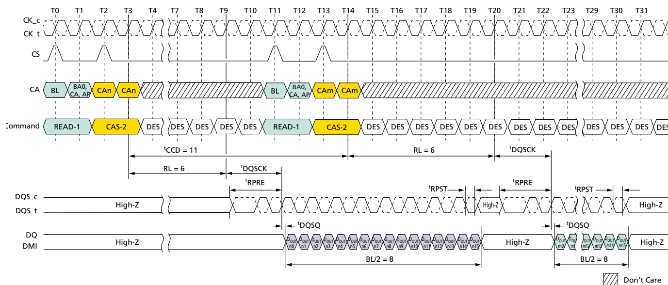
Figure 49: Consecutive READ: t_{CCD} = \text{MIN} + 3 , Preamble = Toggle, 0.5n\text{CK} Postamble
