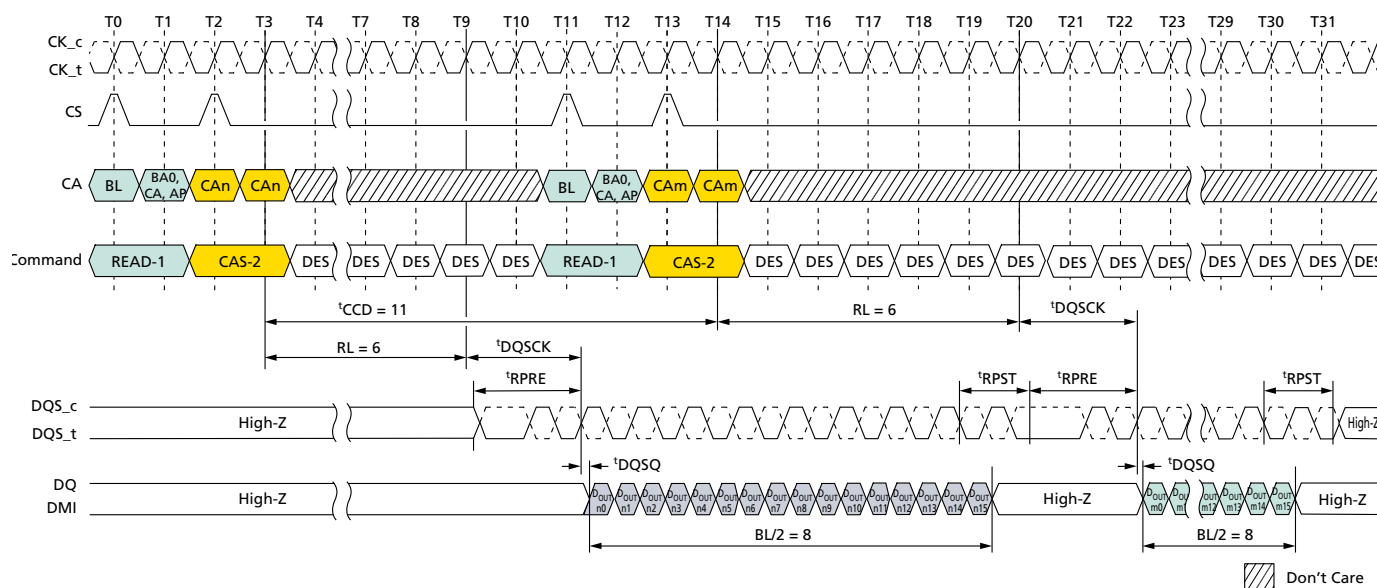
Figure 48: Consecutive READ: t_{CCD} = \text{MIN} + 3 , Preamble = Toggle, 1.5n\text{CK} Postamble
