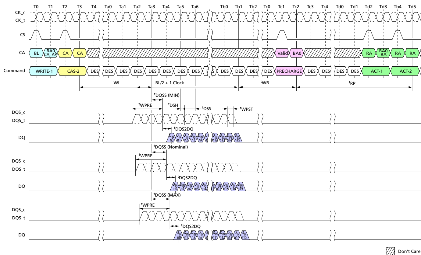
Figure 26: Burst WRITE Operation
