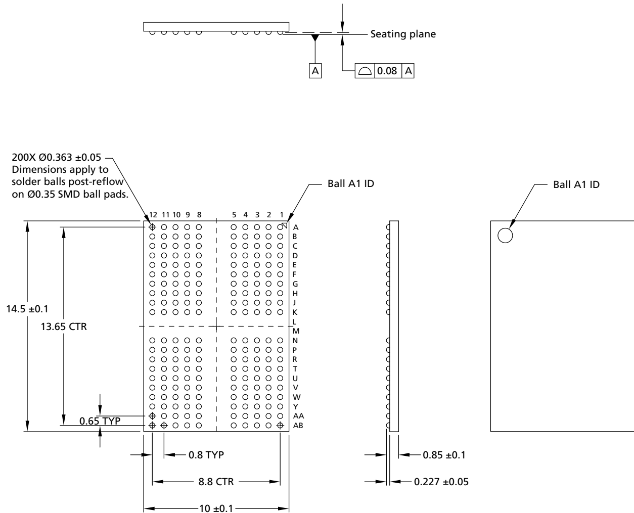
Figure 7: 200-Ball VFBGA – 10mm x 14.5mm (Package Code: DT)
