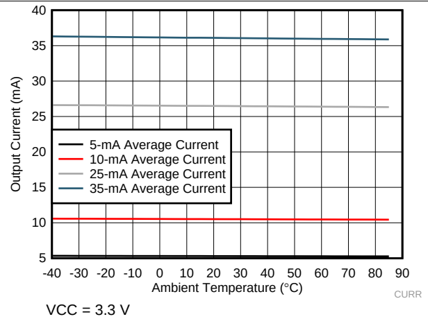
图 3. Output Current vs Temperature
