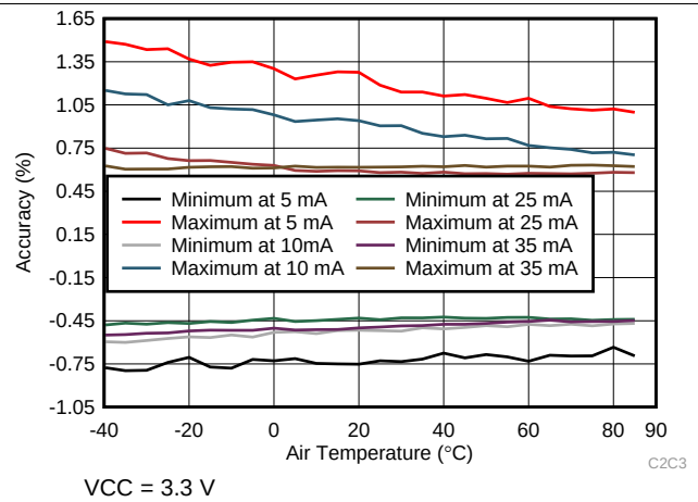
图 5. Channel-to-Channel Current Accuracy
