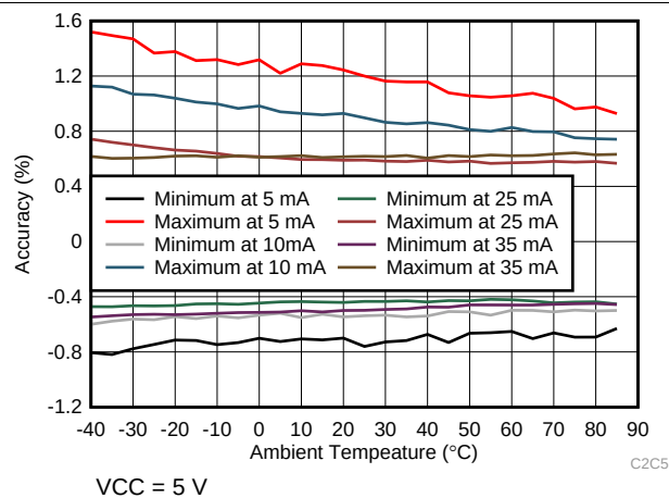
图 6. Channel-to-Channel Current Accuracy vs Temperature
