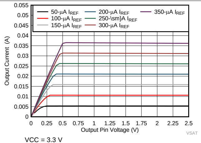
图 7. OUT Pin Voltage vs Current
