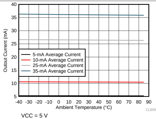
图 4. Output Current vs Temperature
