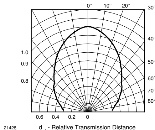
Fig. 13 - Vertical Directivity
