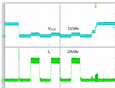
Short Circuit Protection ( V_{IN}=5.0V , V_{OUT}=1.05V , I_O=4A \sim short)
