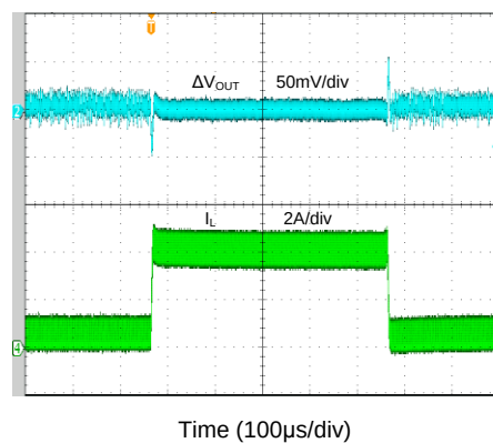
Load Transient ( V_{IN}=5.0V, V_{OUT}=1.05V, I_O=0.4 \sim 4.0A )
