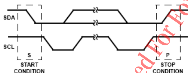
Figure3. START and STOP Conditions
