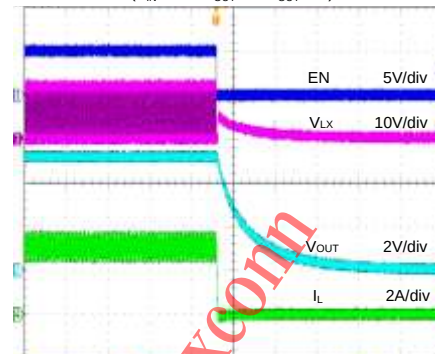
Shutdown from Enable ( V_{IN}=12V , V_{OUT}=5V , I_{OUT}=3A )
