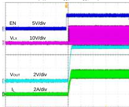
Startup from Enable ( V_{IN}=12V , V_{OUT}=5V , I_{OUT}=3A )
