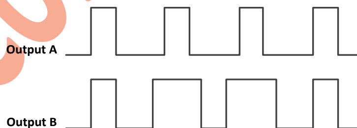
Figure 16. PWM Output Signals in D-BTL Mode
