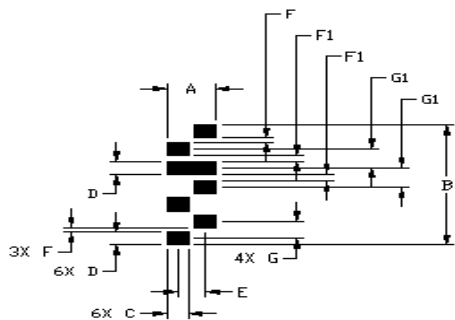
Pad Layout
