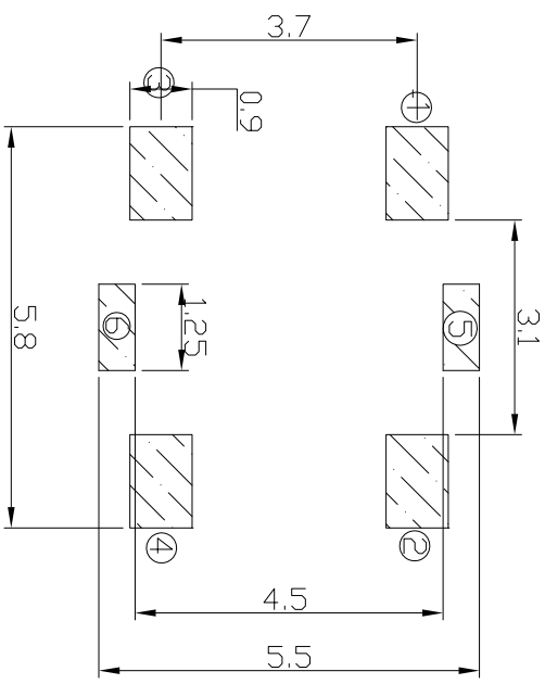
P. C. B LAYOUT
