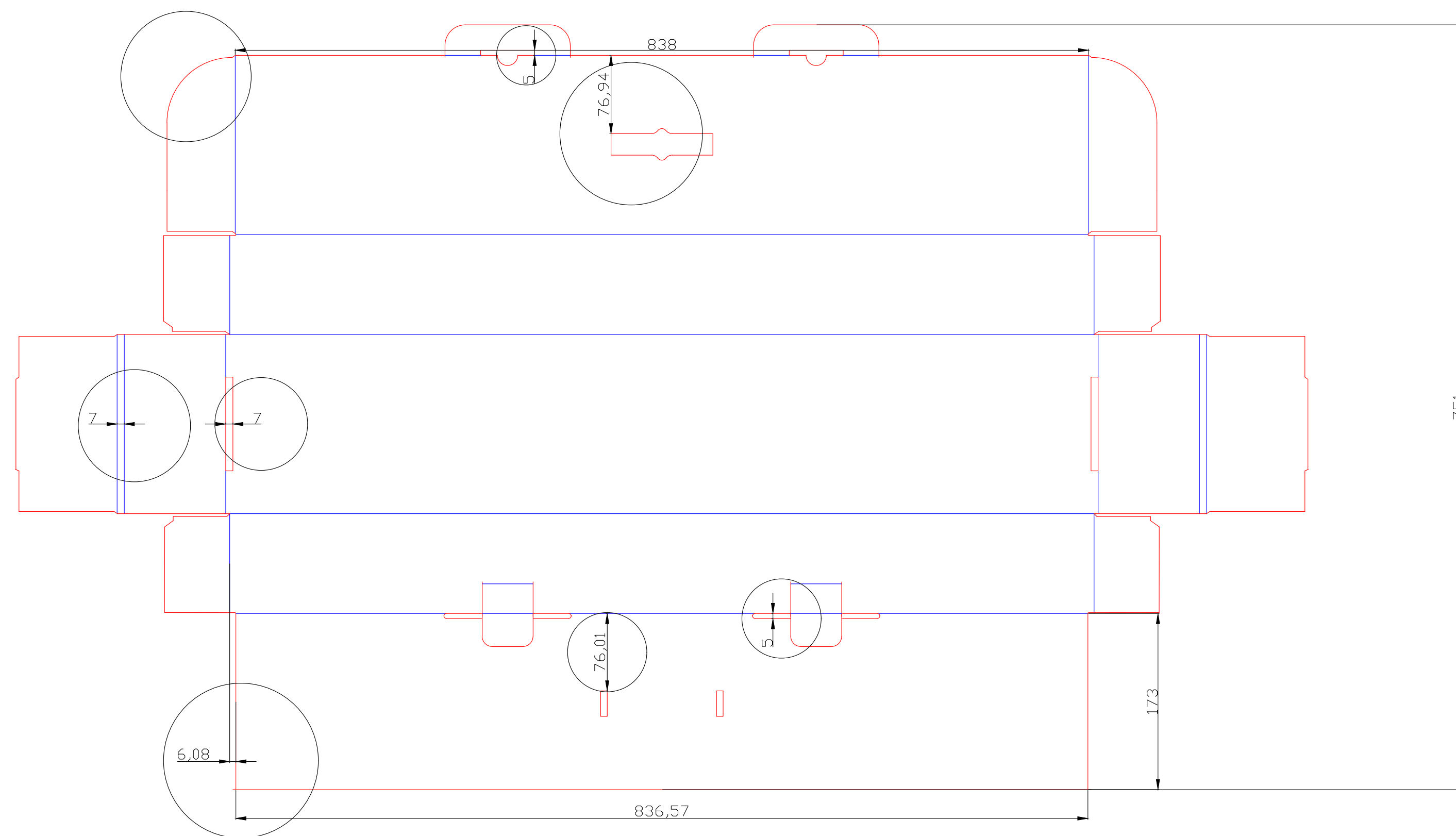
修改过小 细节 Some modifications and enlarged to fit in B flute thickness
