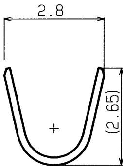
INSULATION BARREL
